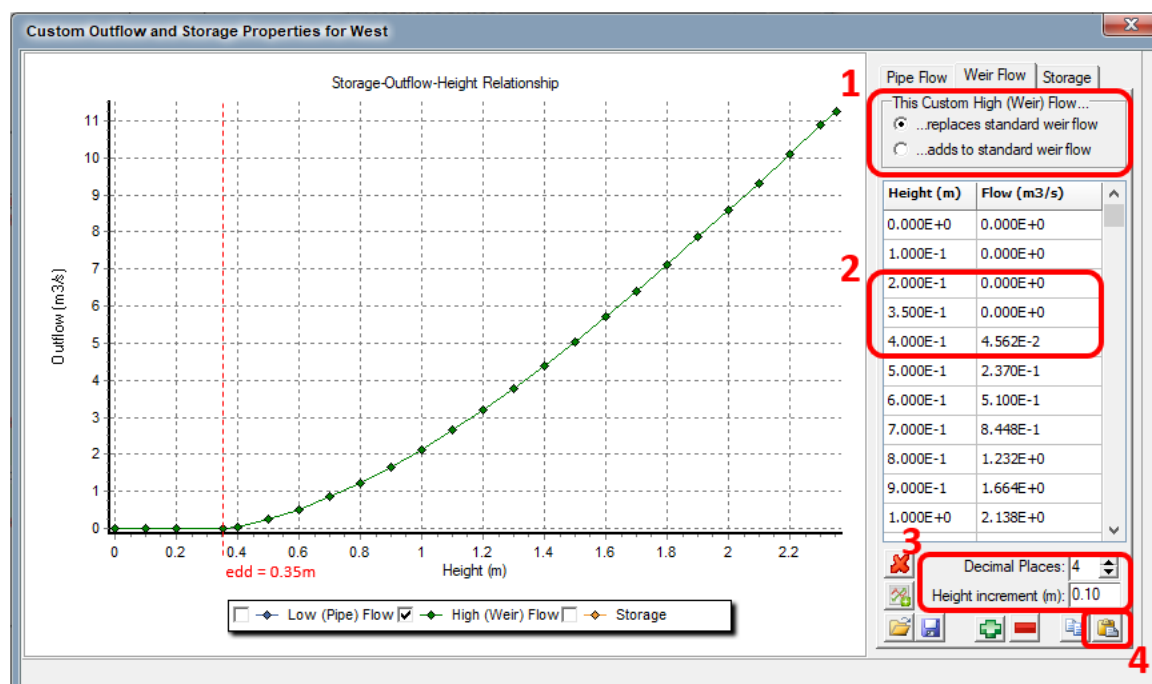
Figure 26 Example stage-discharge relationship for weir flow
