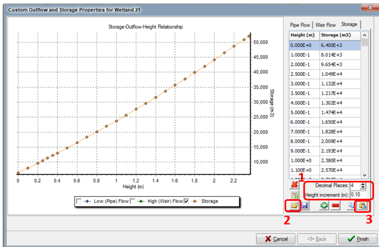
Figure 24 Example stage-storage relationship
