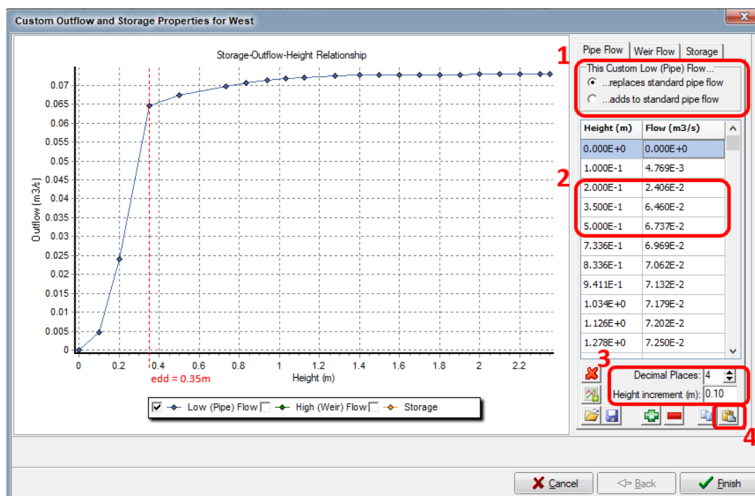
Figure 25 Example stage-discharge relationship for pipe flow
