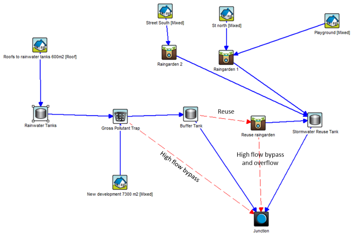
Figure 8 Directing high flow bypasses and overflows to outlet, pumped reuse from a buffer to a raingarden and outflows to a stormwater reuse storage
