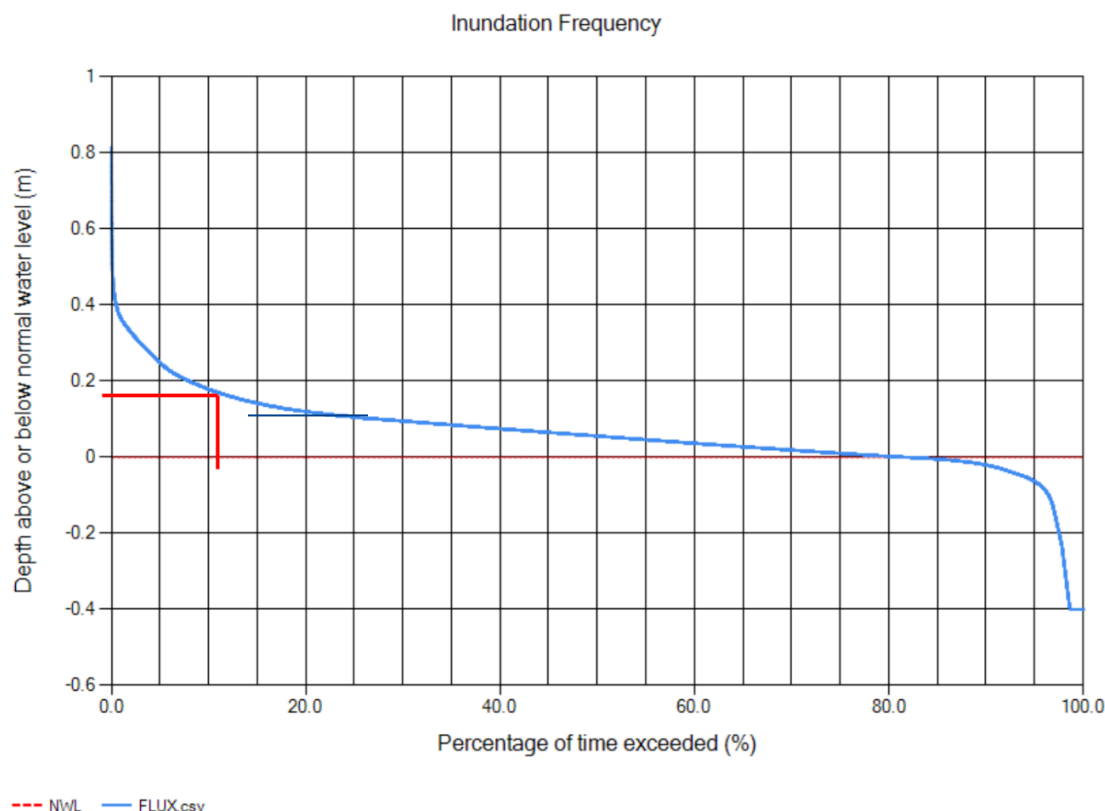
Figure 19 Typical inundation frequency curve for a wetland
