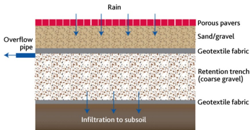
Figure 21 A typical permeable pavement cross section
