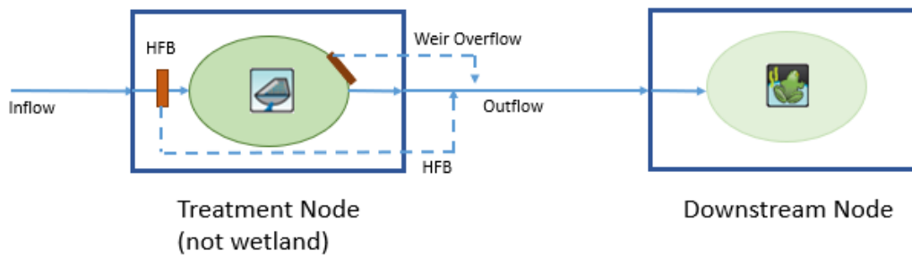
Figure 13 Behaviour of most treatment nodes with high flow bypass upstream (HFB) and weir overflows from downstream end for most treatment nodes
