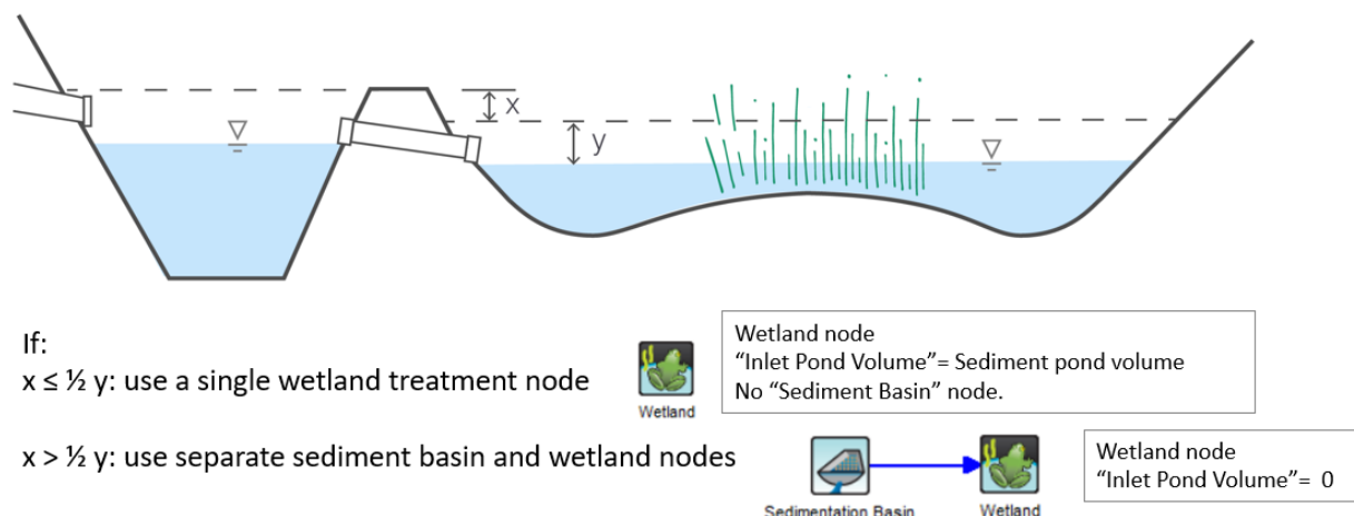
Figure 18 Sediment pond and wetland extended detention levels
